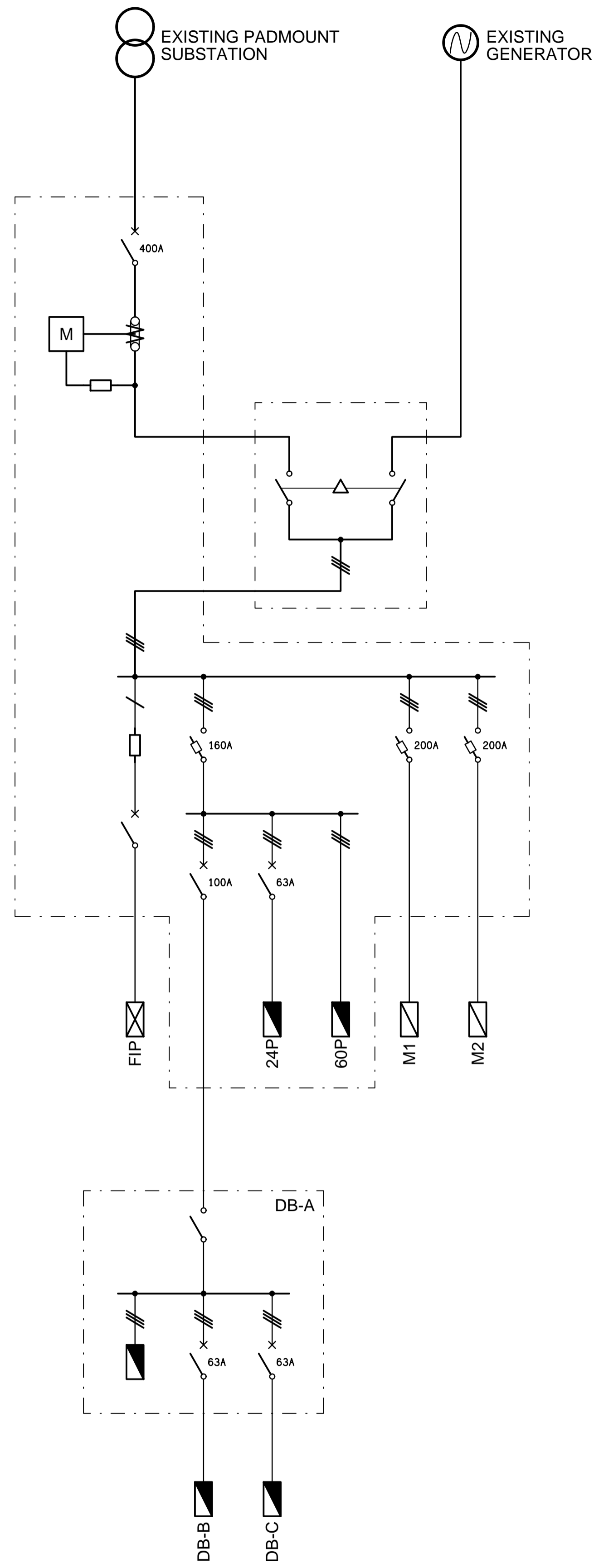
EXISTING POWER SCHEMATIC NOT TO SCALE
