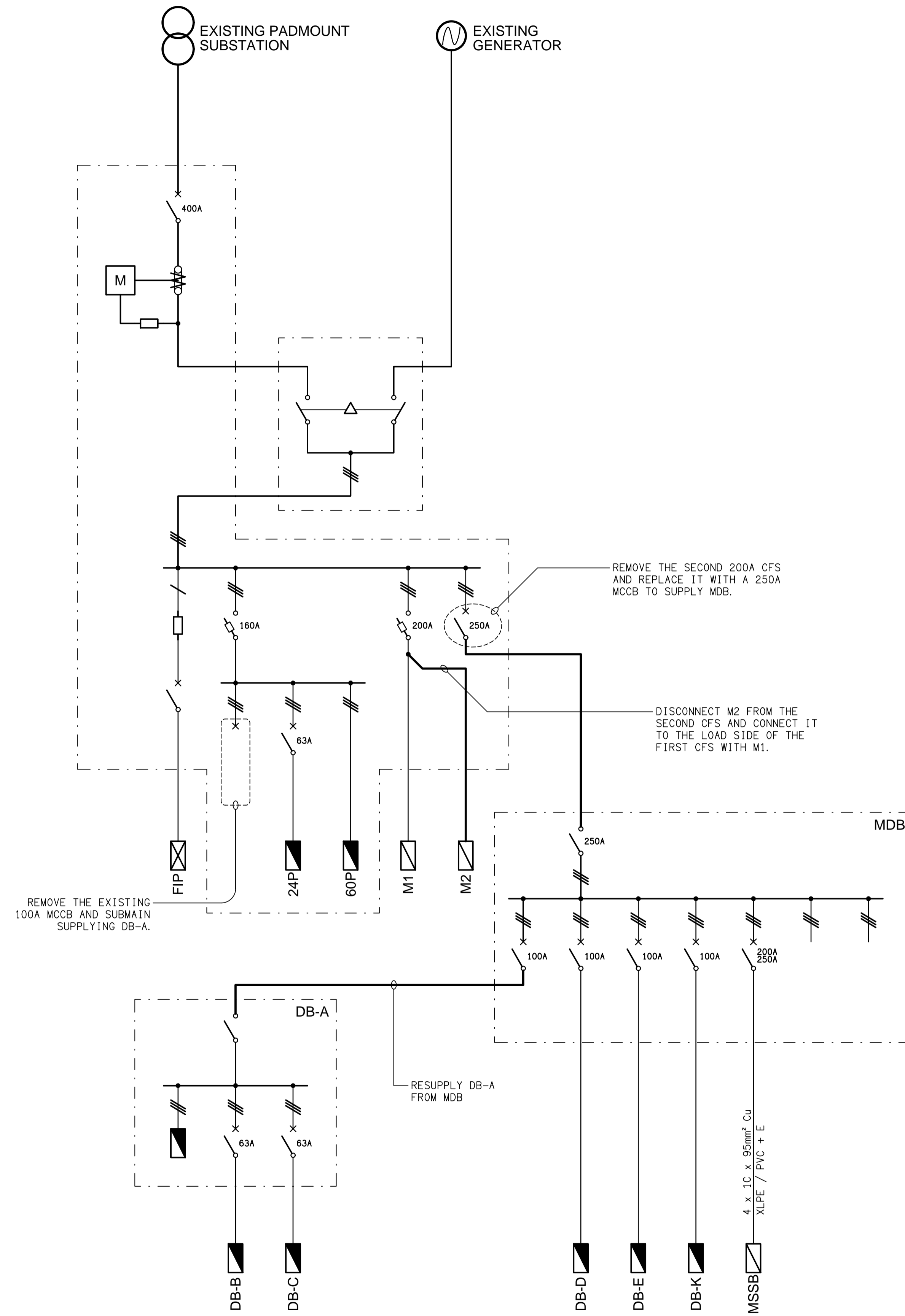
PROPOSED POWER SCHEMATIC NOT TO SCALE
